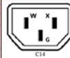
IEC 60320 C13/14 120/240 volt, Single Phase 3 wire, grounding 10 amp
