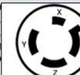
NEMA L15-20 240 volt, 3Ø, three pole, 4 wire, grounding 20 amp
