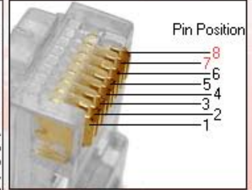
8 Pin 8 Connector (8P8C) (RJ45)
