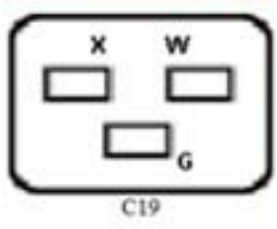
IEC 60320 C19/20 120/240 volt, Single Phase 3 wire, grounding 16 amp
