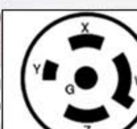
NEMA L21-20 120/208 volt, 3ØY, four pole, 5 wire, grounding 20 amp
