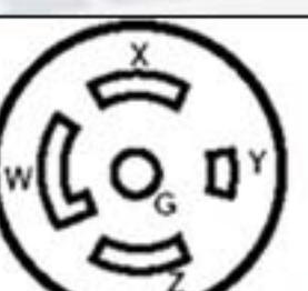
NEMA L21-30 120/208 volt, 3ØY, four pole, 5 wire, grounding 30 amp
