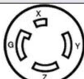
NEMA L15-30 240 volt, 3Ø, three pole, 4 wire, grounding 30 amp
